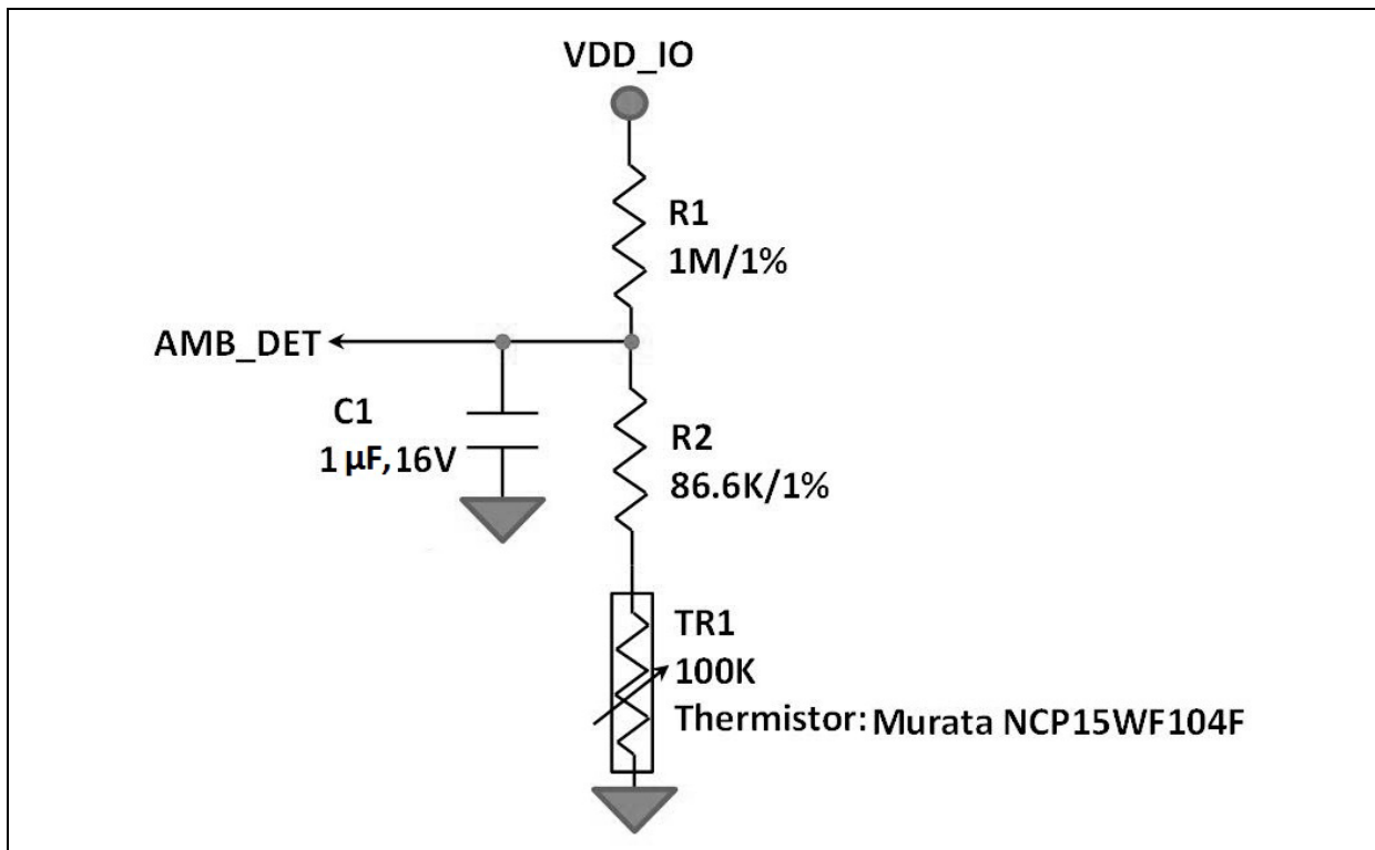
FIGURE 4-3: AMBIENT DETECTION
